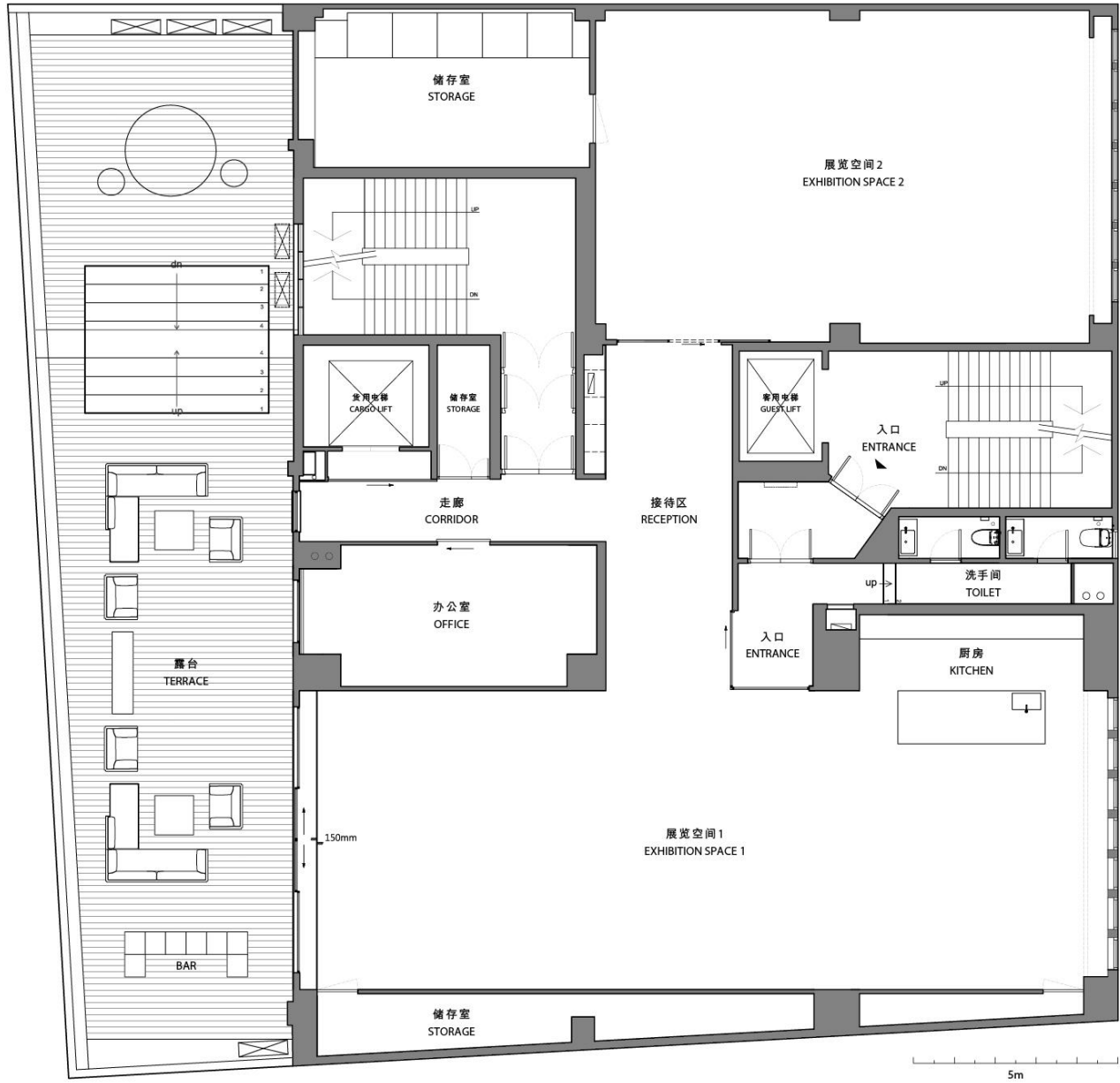
Floor Plan
